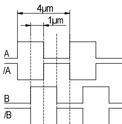
Fig. 2: Output of the quadrature signals
